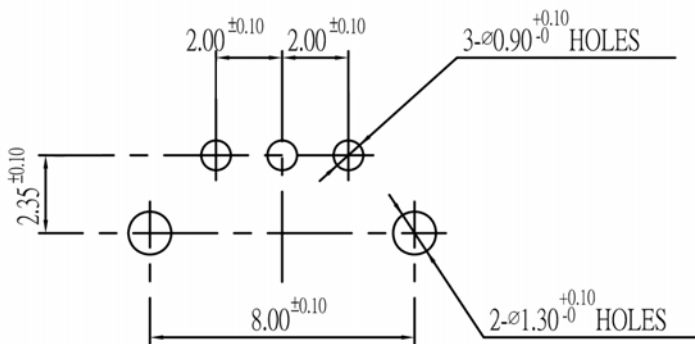
P.C.B. LAYOUT (VIEW FROM THE DIRECTION A)
